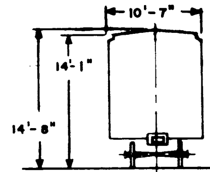
PACIFIC CAR & FDY. CAR-PAK LOADER -9 BELTS
