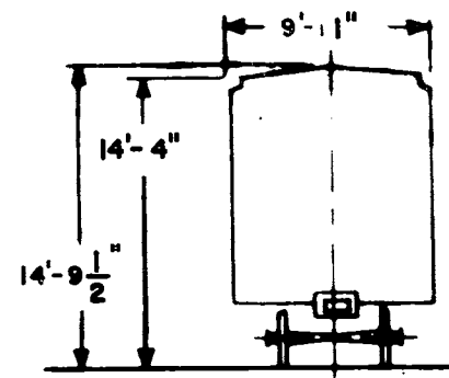
SINGLE SHEATHED VERT. O/S POST
