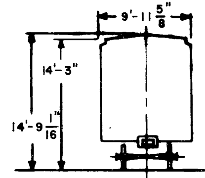
DF-2 BELT RAILS END DOOR
