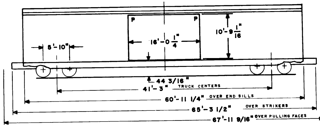
PLATE "C" FREIGHT SAVER CUSHION
