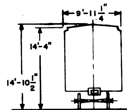
SINGLE SHEATHED VERT. OUTSIDE POST
