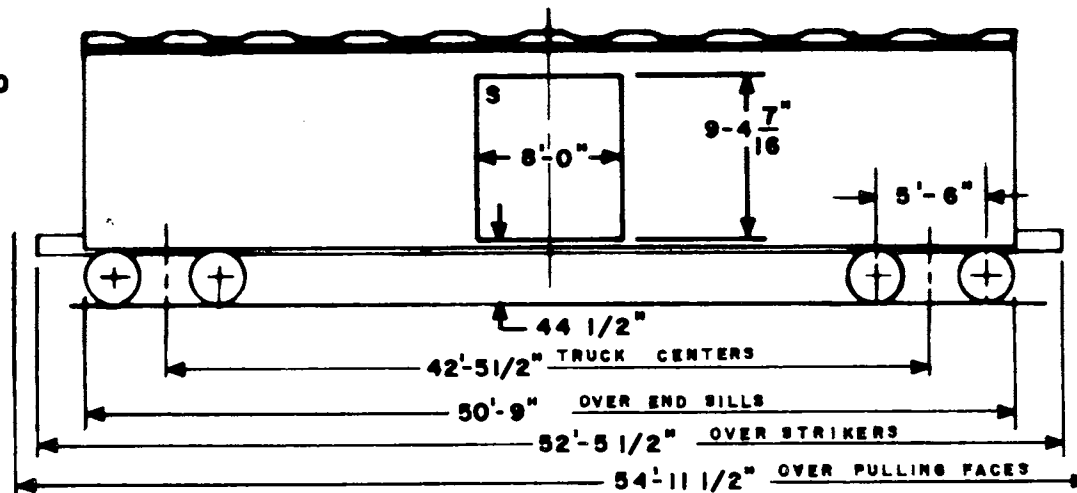
PACIFIC CAR & FDY. CAR-PAK LOADER -9 BELTS
