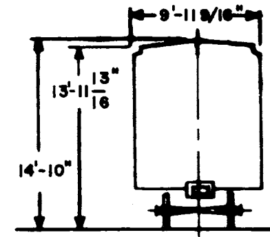
HIDE &amp; TANKAGE LOADING
