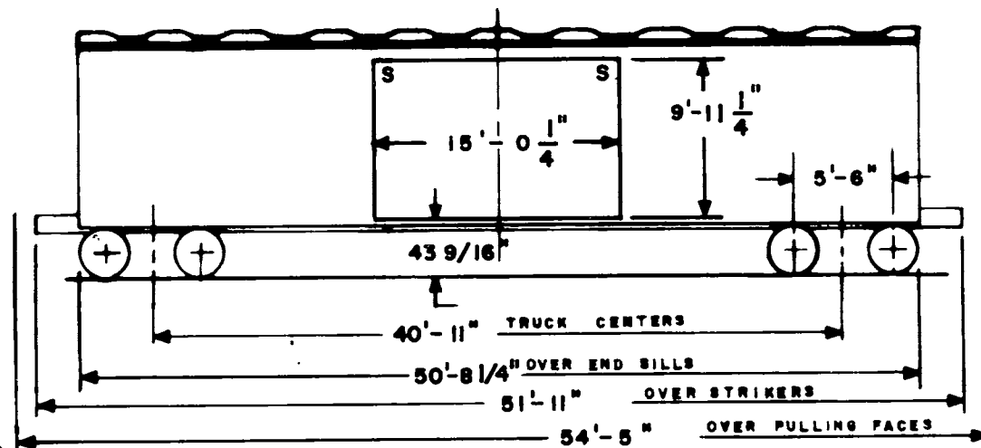
SINGLE SHEATHED VERT. O/S POST
