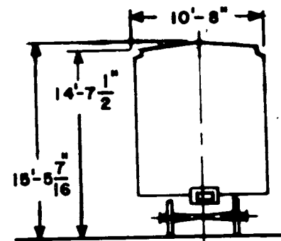
FREIGHT MASTER CUSHION 12" TRAVEL (SINGLE SHEATHED)
