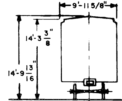
NAT'L. 3-C CUSHION 24" TRAVEL HEATER HOOKS IN CEILING
