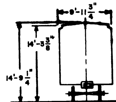
(4) DF-2 BELT RAILS FREIGHT SAVER 20-B CUSHION UNIT.
