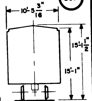
PLATE "C" FREIGHT SAVER CUSHION
