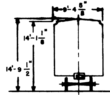
HIDE &amp; TANKAGE LOADING
